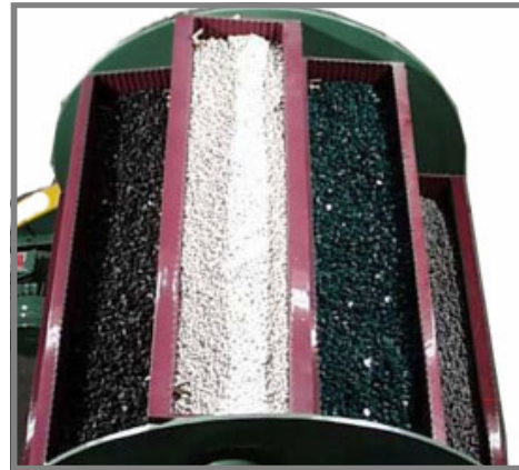
TOP VIEW OF TUBS SHOWS VARIOUS MEDIA: FAST CUT CERAMIC, PLASTIC MEDIA TO REFINE R.M.S., PORCELAIN TO POLISH AND CORN COB MEDIA FOR FINAL PART DRYING STEP. NOTE: COMPARTMENT DIVIDERS CAN BE ADDED TO SEPARATE PARTS.
